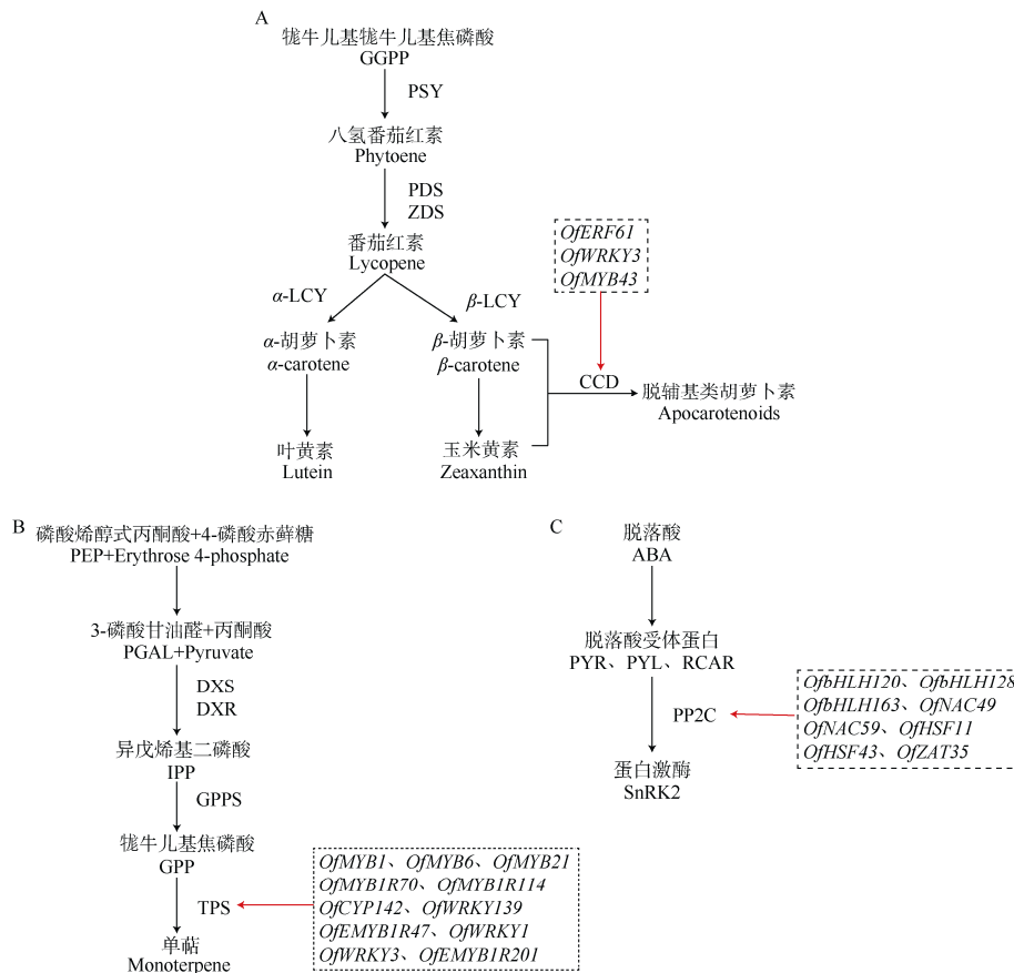
图 1 桂花相关性状信号通路。A: 花色; B: 花香; C: 低温; PSY: 八氢番茄红素合酶; PDS: 八氢番茄红素去饱和酶; ZDS: \zeta -胡萝卜素去饱和酶; \alpha -LCY: 番茄红素 \alpha -环化酶; \beta -LCY: 番茄红素 \beta -环化酶; CCD: 类胡萝卜素切割双加氧酶; DXS: 1-Deoxy-D-xylulose-5-phosphate synthase; DXR: 1-Deoxy-D-xylulose-5-phosphate reductoisomerase; GPPS: Geranyl pyrophosphate synthase; TPS: Terpene synthase; PYR: Pyrabactin resistance; PYL: Pyrabactin resistance-like; RCAR: Regulatory component of ABA receptors; PP2C: Type 2C protein phosphatases。
